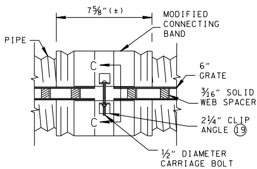
MODIFIED CONNECTING BAND TOP VIEW
