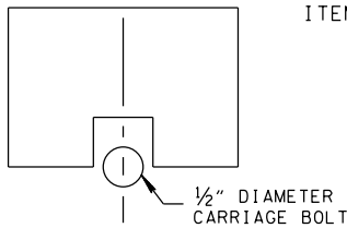
GAP PLATE (OPTIONAL) MAY BE PLACED DIRECTLY OVER BAND BOLT TO PROVIDE CONTINUOUS FORM FOR GROUTING.
