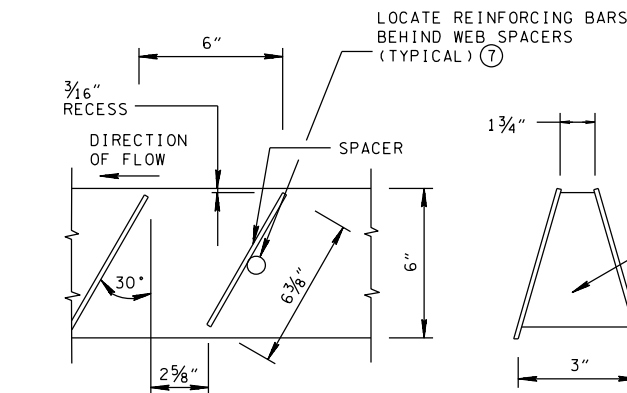
SLANTED WEB SPACERS DETAILS SIDE VIEW (FOR USE WITH TRAPEZOIDAL GRATES ONLY)
