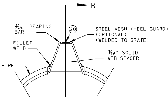
ALTERNATE TRAPEZOIDAL GRATE DETAIL WITH MESH (SECTION A-A)
