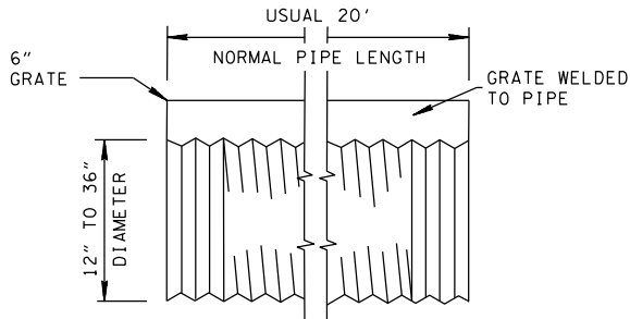
TYPICAL PIPE SECTION
