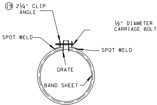
MODIFIED CONNECTING BAND END VIEW (SECTION C-C)
