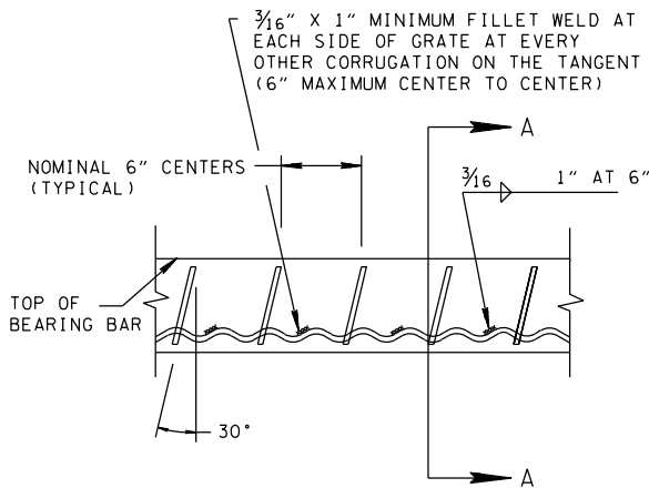
GRATE (BEARING BAR) WELDING DETAIL (WITH SLANTED WEB SPACERS)
