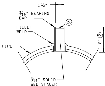
STANDARD PARALLEL (VERTICAL) SIDE GRATE DETAIL (SECTION A-A) (WITH VERTICAL WEB SPACERS)
