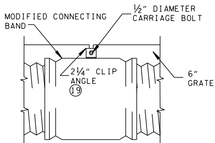
MODIFIED CONNECTING BAND SIDE VIEW
