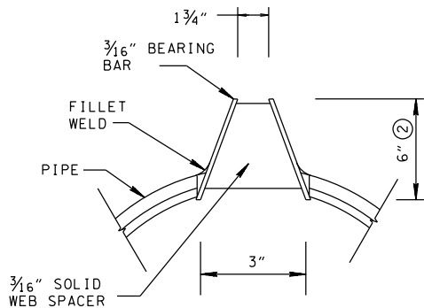
ALTERNATE TRAPEZOIDAL GRATE DETAIL (SECTION A-A)
